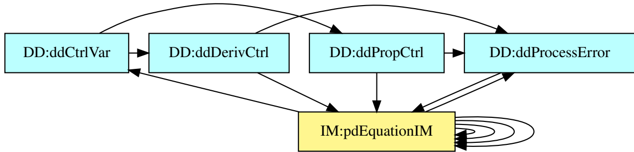
Figure 5: TraceGraphRefsRef
