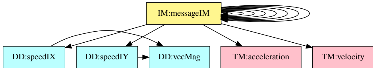
Figure 5: TraceGraphRefsRef
