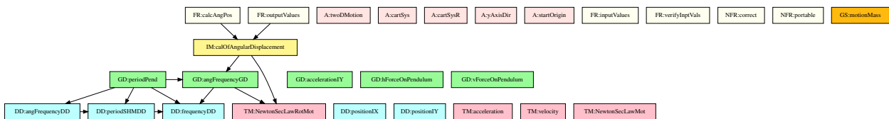
Figure 7: TraceGraphAllvsAll
