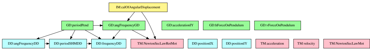
Figure 5: TraceGraphRefsRef
