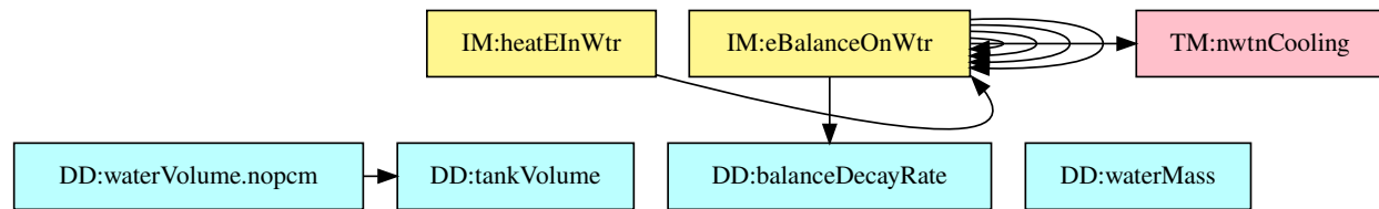
Figure 5: TraceGraphRefsRef
